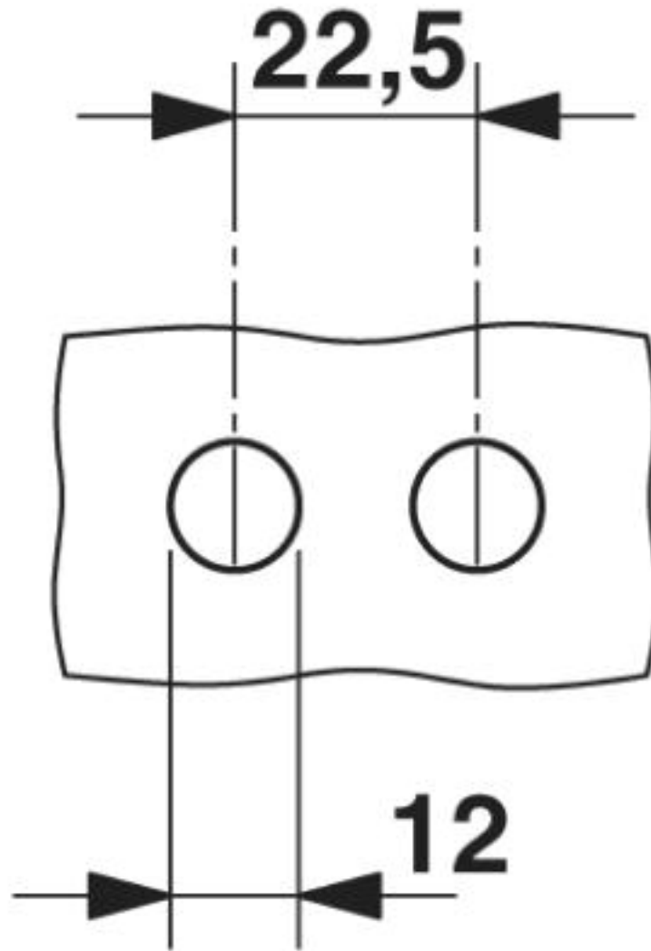
Dimensional drawing
